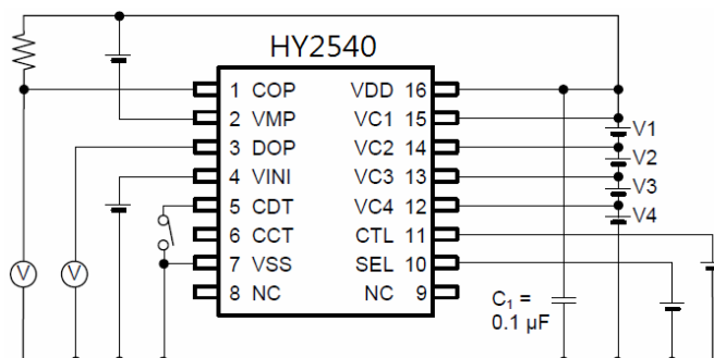
Test Circuit 2
