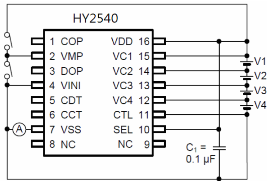
Test Circuit 1
